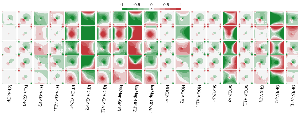
Figure 3: Visualization of local errors. Each image represents the difference between the prediction and ground-truth over individual outputs of one test example in Poisson-II .
