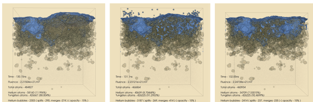
Figure 1: Snapshots around a time the tungsten surface is pushed upward by a over-pressurized helium bubble (left), then recoils as the bubble bursts (center, right). In each snapshot, the tungsten voids are indicated in blue, helium bubbles in gray, and the extracted statistics and bubble evaluation details are also displayed. Here, the simulation box is \approx 20 nm wide.
