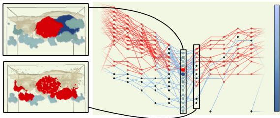
Figure 4: A tracking graph [WCBP12] (right) visualizing the evolution of helium bubbles around the time one helium bubble bursts, same as in Figure 1. Within the graph, each set of nodes in a vertical column represents helium bubbles in one timestep and their evolution are shown as a collection of feature tracks that merge and/or split. The top left and bottom left images visualize the helium bubbles (colored by size using a blue color map) and tungsten voids (in beige) for two timesteps. The bubble that bursts and its evolution is highlighted in ‘red’. For simplicity, only bubbles with size > 500 atoms are visualized.
