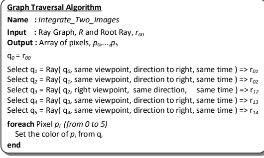
(a) Pseudo-coded graph traversal algorithm
