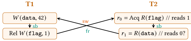
Figure 2. Message passing in C. The release-acquire pair creates an sw edge. If the data read sees the stale value, fr closes a cycle with hb C , forbidden by C’s coherence axiom.
