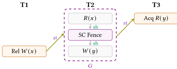
Figure 5. Fence context sharing. The dashed box marks the fence context G = (R(x), \text{SC Fence}, W(y)) .
