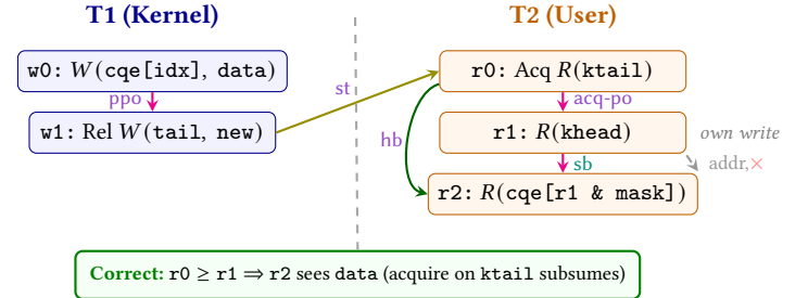
Figure 11. The io_uring completion queue under the compound model. The kernel writes a CQE and releases the tail ( w0-w1 ). The user acquires the tail ( r0 ), reads the head ( r1 , its own bookkeeping), and dereferences ( r2 ). The hb chain w0 \xrightarrow{ppo} w1 \xrightarrow{st} r0 \xrightarrow{hb} r2 guarantees r2 sees the kernel's write. The address dependency from r1 to r2 (greyed, \times ) is formally redundant.
