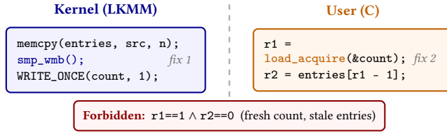
Figure 1. The kcov_remote cross-boundary bug. Initially count = 0 and entries[] is zeroed; src holds nonzero data. The figure shows the first append, so the count update writes 1. load_acquire abbreviates __atomic_load_n(..., __ATOMIC_ACQUIRE) . Neither fix alone suffices: smp_wmb() on the kernel side has no effect if the user-side load is C-relaxed, and an acquire load on the user side has no effect if the kernel's stores are unordered under LKMM. The bug is closed only by a matched pair across the boundary—precisely the contract of our C/LKMM compound memory model.
