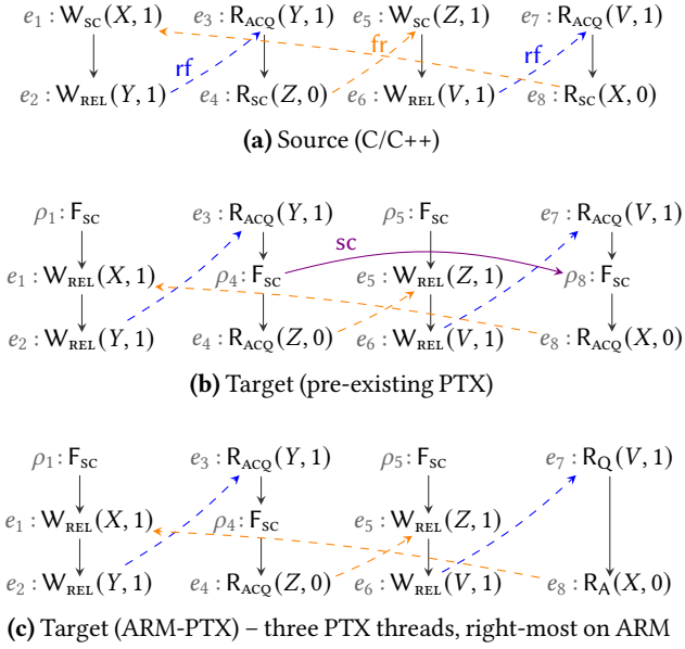
Figure 7. Executions of the example programs in Figure 2. scoped-C/C++ forbids the outcome a=1, b=0, c=1, d=0 . ARM-PTX must thus also forbid the outcome in the target execution to ensure correctness of the existing mapping schemes.
