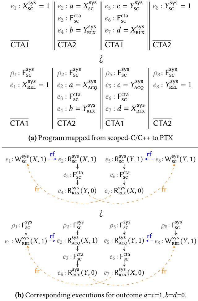
Figure 10. Program mapped from scoped-C/C++ to PTX with its executions, with F_{SC}^{cta} s in different CTAs.
