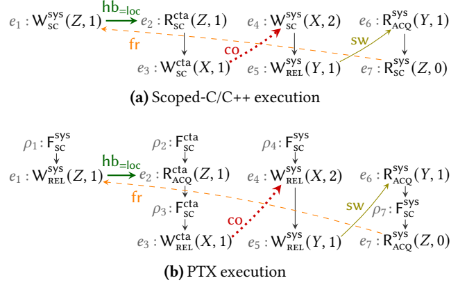
Figure 6. Execution of the source scoped-C/C++ and the generated PTX programs from Figure 3. The source scoped-C/C++ execution forbids the outcome a=b=1, c=0, X=2 but the PTX execution allows it (under the pre-existing PTX model).
