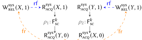
Figure 9. Execution graph of IRIW-F program with outcome a=c=1, b=d=0 .
