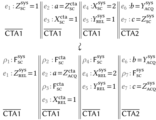
Figure 3. An incorrect compilation from scoped-C/C++ to PTX. The outcome a=b=1, c=0, X=2 is forbidden in the source program but allowed in the generated PTX program.
