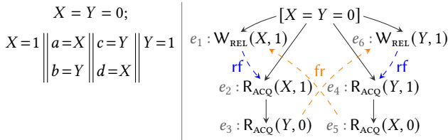
Figure 8. IRIW-RA program (with release-writes and acquire-reads) and its a=c=1, b=d=0 execution. (All sys-scoped)
