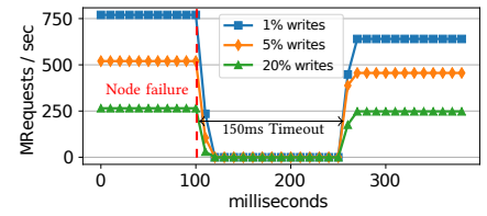
Figure 9. HermesKV under failure. [Uniform traffic, 5 nodes, timeout=150ms]
