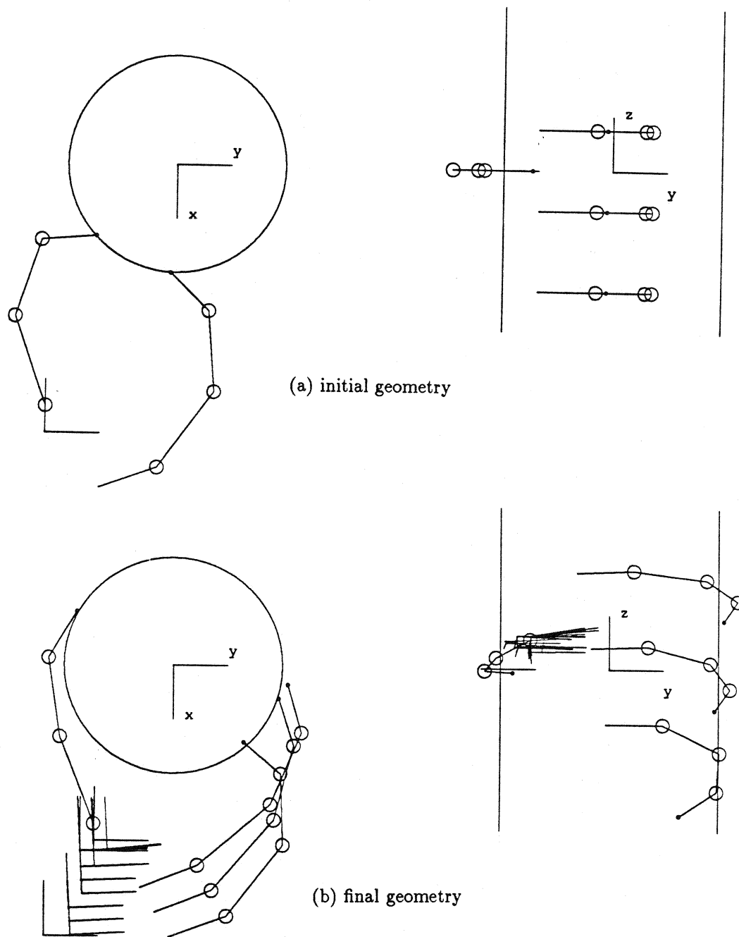
Figure 10: The synthesis of a four fingered grasp for the Utah/MIT hand
