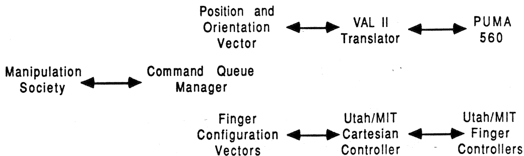
Figure 11: The Control Structure for a Manipulation Test Bed
