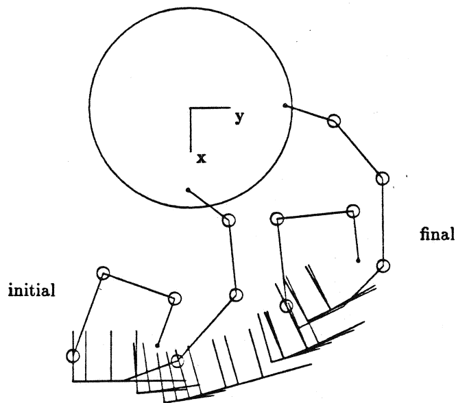
Figure 7: The Conditioning of One Finger for an Isotropic Wrench + F_y
