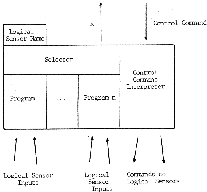
Figure 2. Logical Sensor Specification with Control
