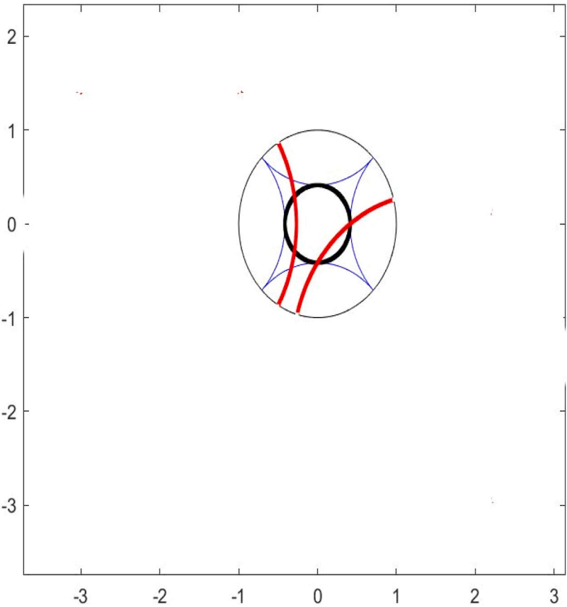
Fig. 13. Chops for Modus Ponens.
