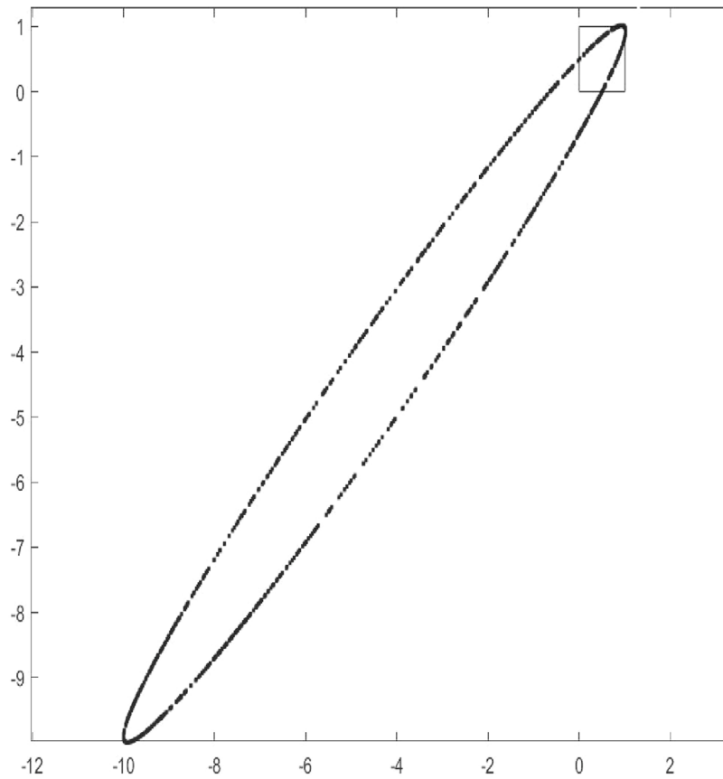
Fig. 3. Example 2-D MVE Showing Major Semi-Axis in Direction of Solution.
