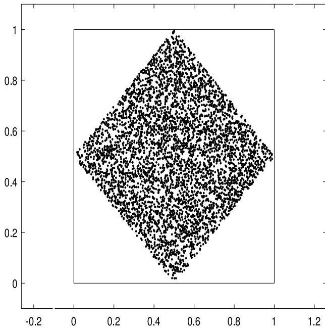
Fig. 2. Example 2-D Feasible Region Resulting from Chopping all Corners of H_2 .
