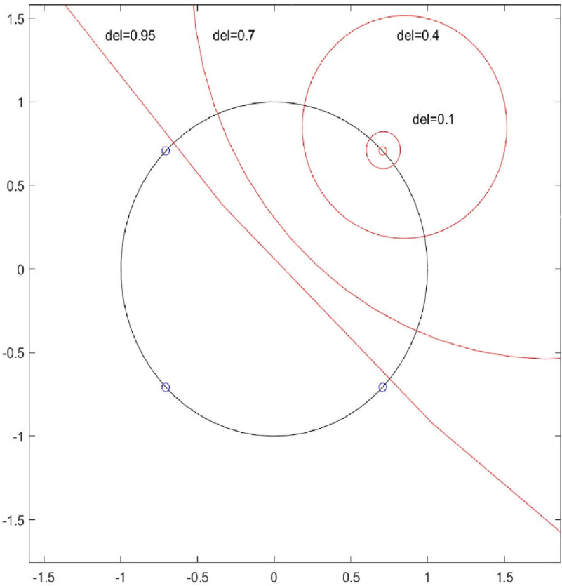
Fig. 12. The Impact of \Delta on Chop Distance from Non-Solution Vertices.
