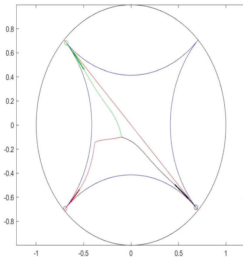
Fig. 17. The Paths for the Barrier Method finding Solutions in a 2D Problem.
