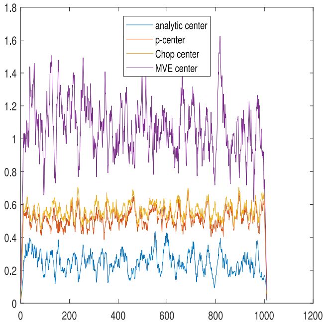
Fig. 4. Error of Approximation Methods: Analytic Center (blue), P-Center (red), Chop center (mustard), MVE center (purple). (For interpretation of the references to color in this figure legend, the reader is referred to the web version of this article.)
