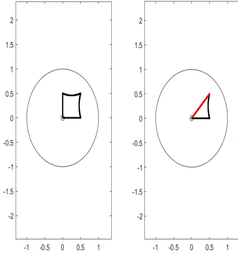
Fig. 9. Representing the Complete Feasible Region as a Square in the Poincaré Disk. The left side is the complete feasible region, while the right side shows the feasible region when (0, 1) is not a truth assignment that satisfies the sentence.
