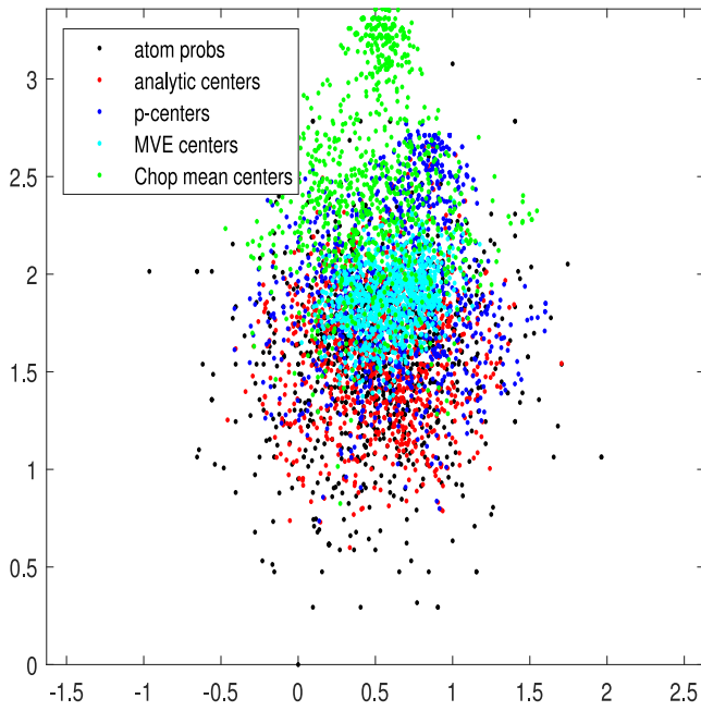
Fig. 5. The center distributions.
