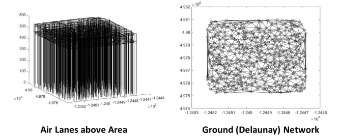
Fig. 12. Lanes Constructed from Delaunay Triangulation (left: airways; right: ground network).
