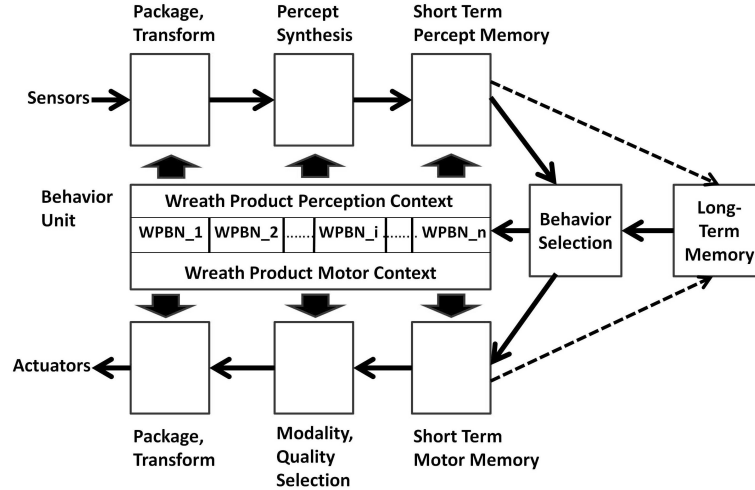
Figure 5: Lower Level Layout of Cognitive Process.
