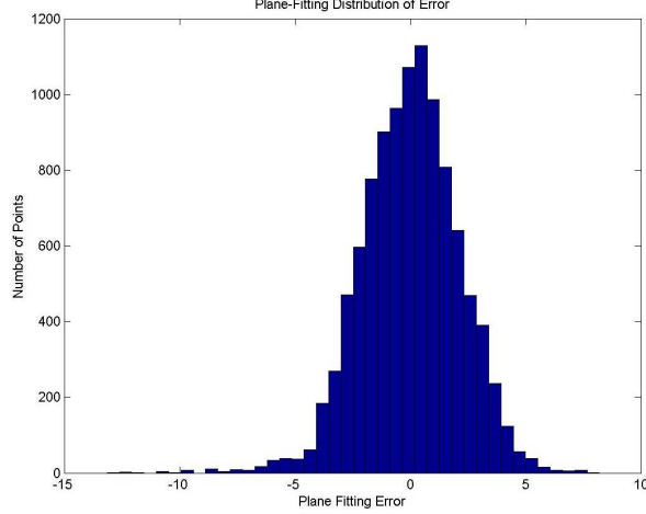
Figure 13: Error Distribution in Plane-Fitting for Kinect Data.
