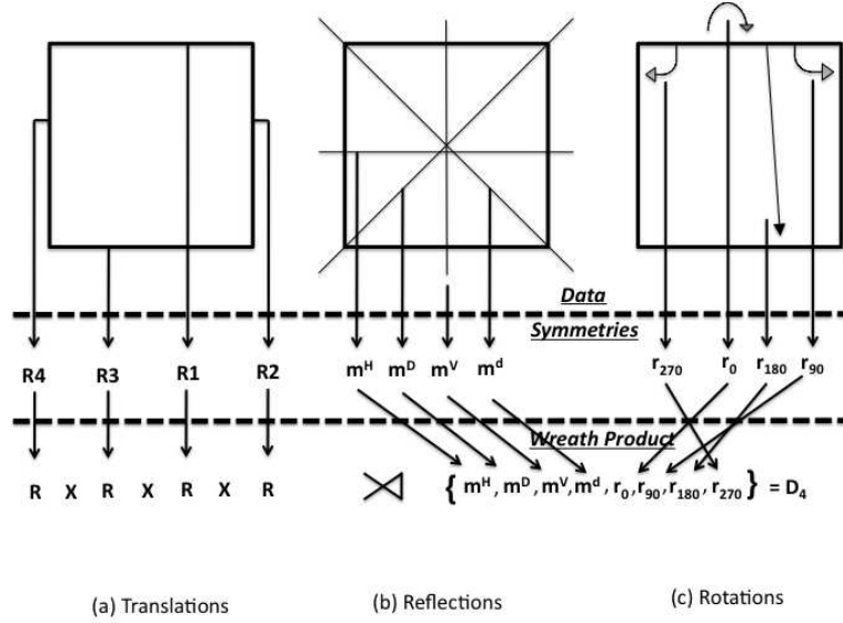
Figure 6: Symmetry Detection in Image of a Square.
