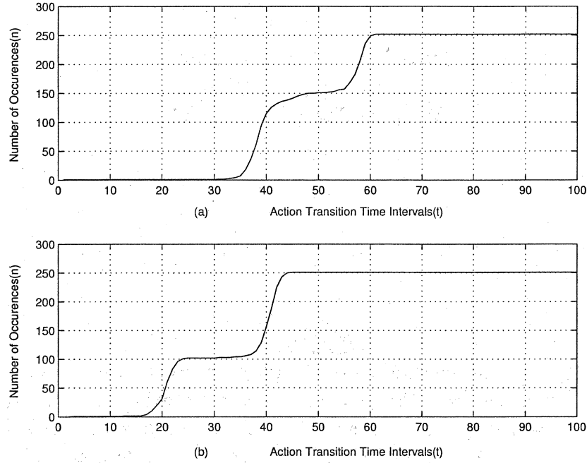
Figure 15: Cumulative Histogram of Action Transition Intervals with Light Context, for (a) Rest⇒Explore Transition and (b) Explore⇒Rest Transition.
