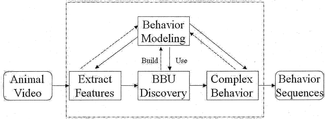
Figure 2: Work-flow for Video Based Behavior Analysis.
