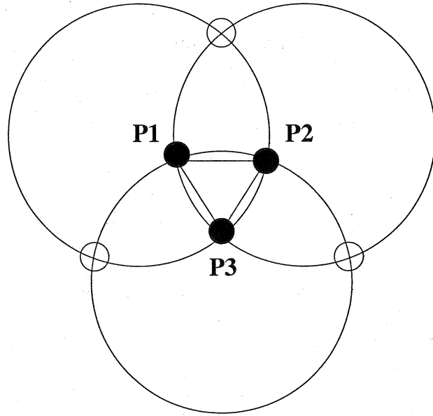
Fig. 2. Geometry of Sensor Range Intersection.
