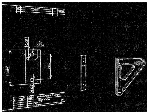
Figure 10. Side view of part from drawing being registered with 3D model.
