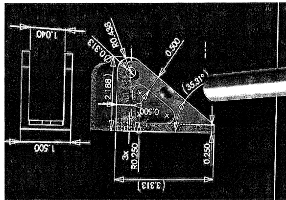
Figure 3. An engineering drawing directly compared with a reconstructed CAD model and a point cloud. The point cloud is registered with the CAD model. Also shown is the tracked wand represented by a gray cylinder.
