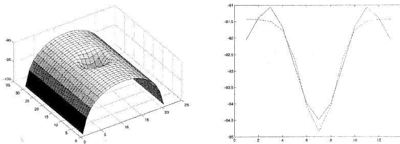
Figure 15: The left image is the surface of a synthetic dented cylinder. The dent shape is Gaussian. The right image is a cross section of the dent fitted with a separable Gaussian. The fitting error is 0.0971.
