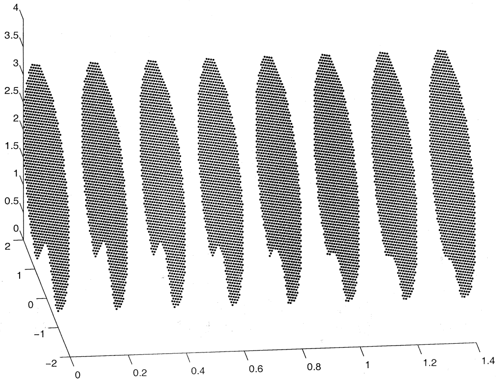
Figure 14: Gouged Surface.
