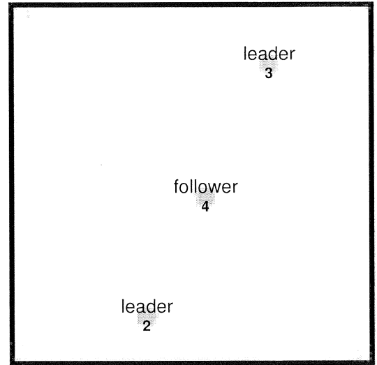
Fig. 3. Final resolution of S-elements in Example 1 after Node 1 has been removed
