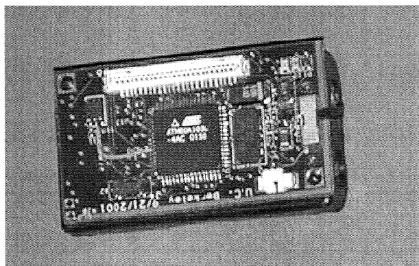
Fig. 1. Berkeley Mote
