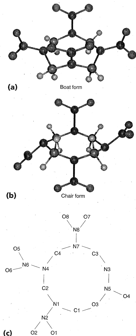
Figure 6. The HMX molecule: (a) boat form, (b) chair form, and (c) stable 10-sided ring intermediate form.
