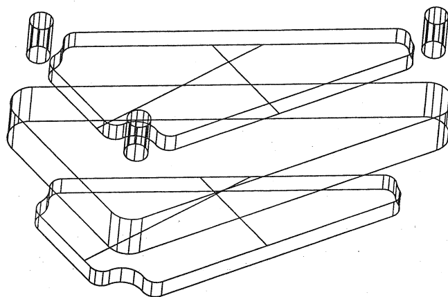
Fig. 17. Exploded view of the features making up the reverse engineered shock plate.
