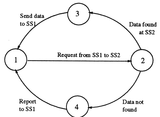
Figure 4: Data request protocol.
