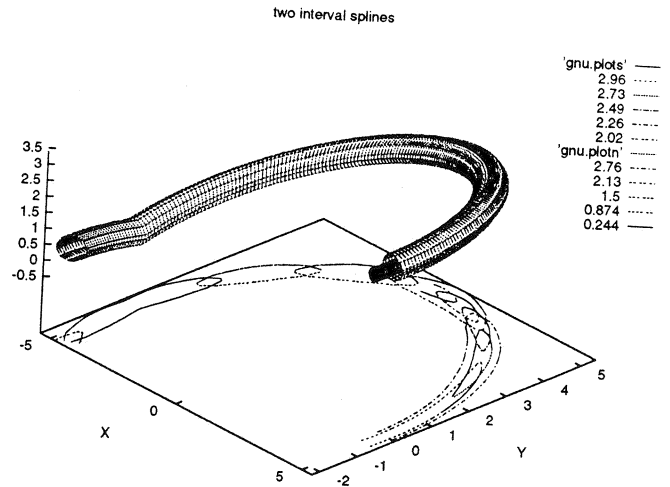
Figure 5: Open torii with a vertical deformation
