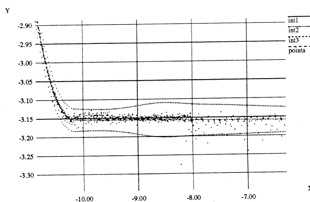
Figure 8: The points from the scanner and the computed offset surface: a detail of the outer pocket
