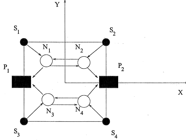
Figure 1: Artificial Amoeba
