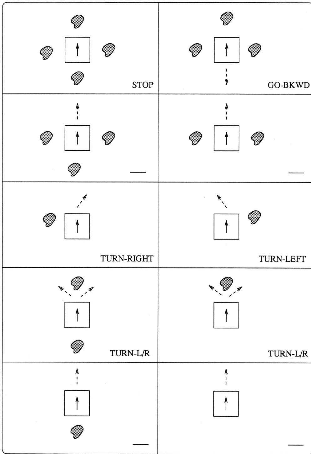
Figure 8: The reaction control when the system state = FORWARD .
