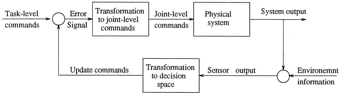
Figure 1: Closed loop control system.
