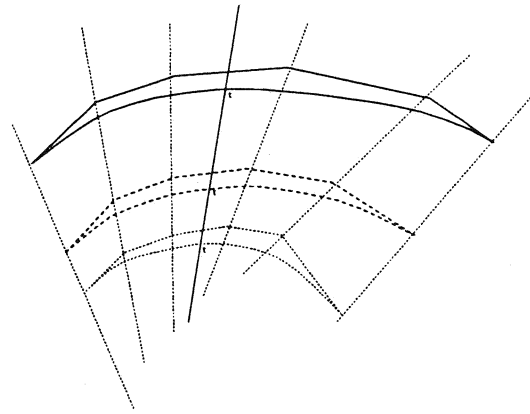
Figure 2: One Interval Spline
