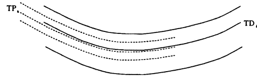
Figure 3: TP_a \subset TP_d
