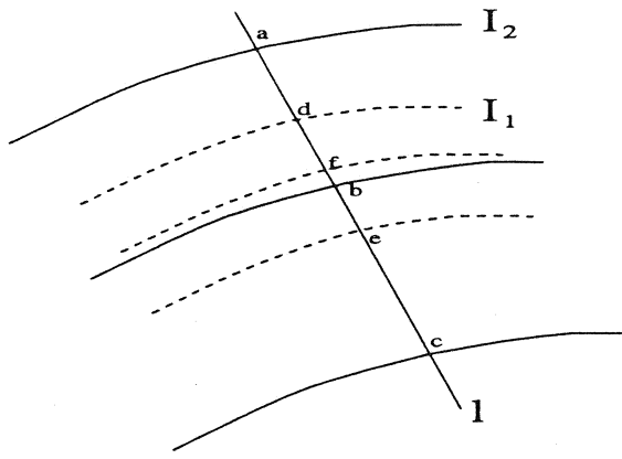
Figure 4: Included Interval Spline
