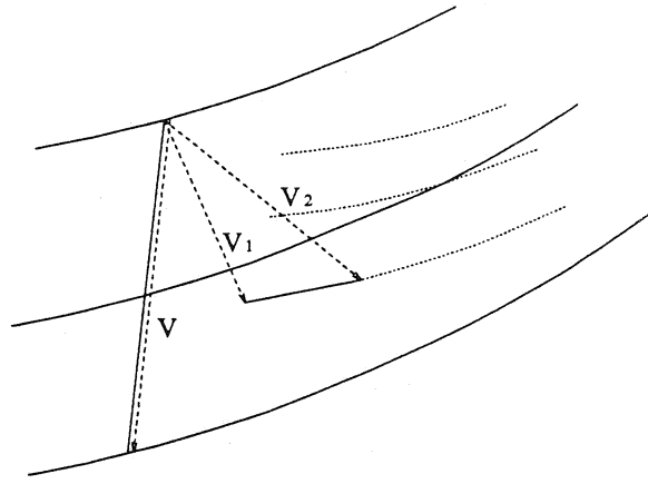
Figure 5: Two Interval Splines
