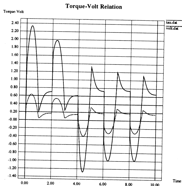
Figure 3: The Relation Between the Torque and the Voltage.
