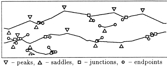
Figure 4: Extracted features
