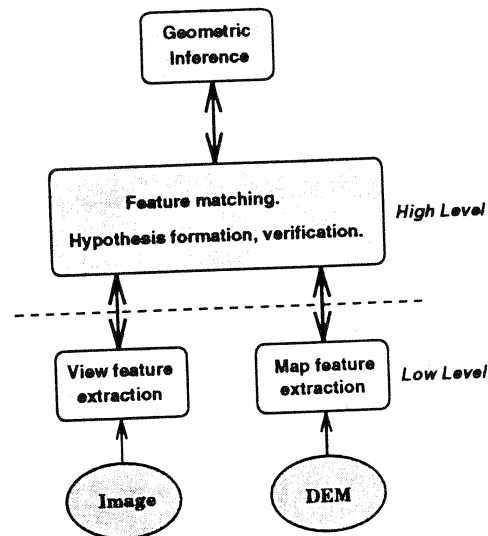
Figure 8: Interaction of high-level and low-level subsystems.
