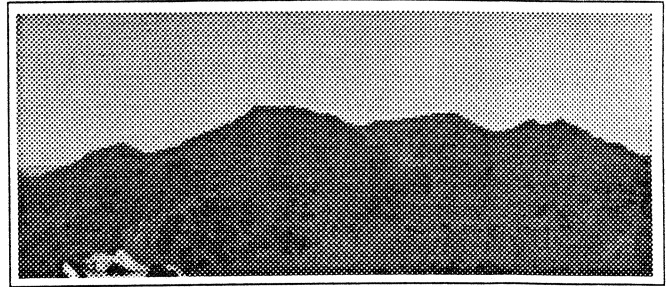
Figure 1: Original Image
