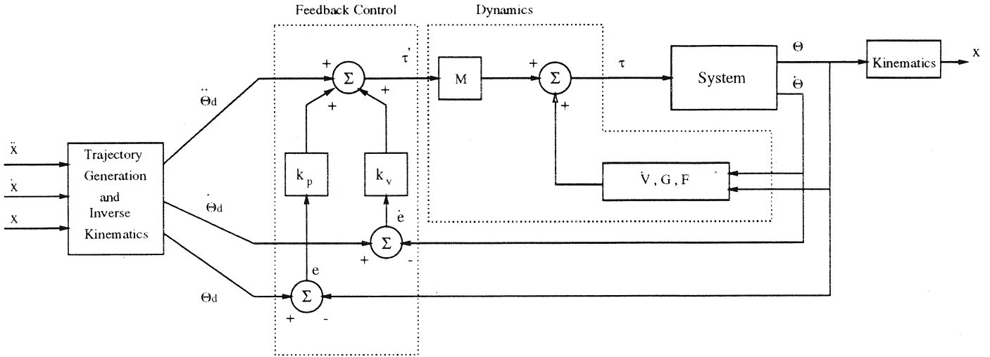
Figure 5: Block diagram of the Controller of a Robot Manipulator.
