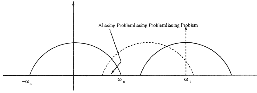
Figure 6: Sampling Theory and the Aliasing Problem.
