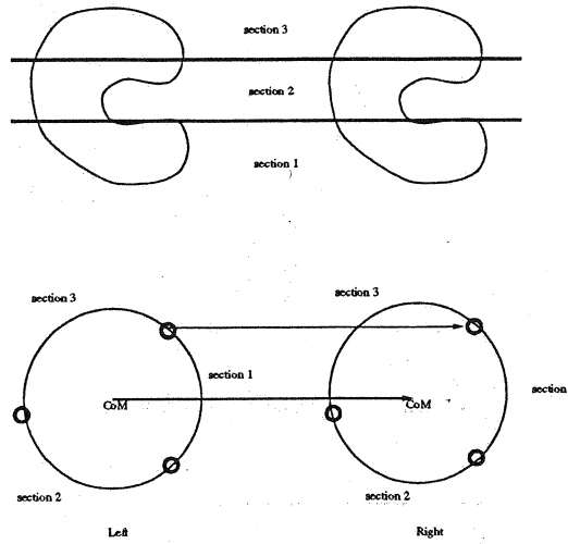
Figure 18: Region Splitting Algorithms
