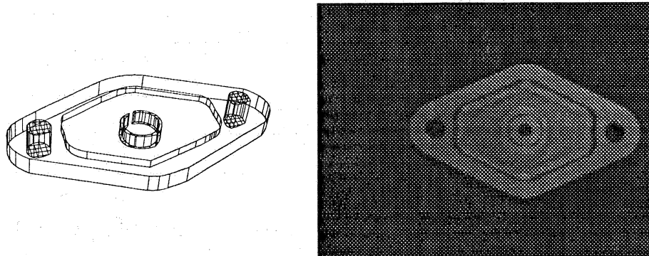
Figure 30: A rough Alpha 1 surface model extracted from the machine vision
