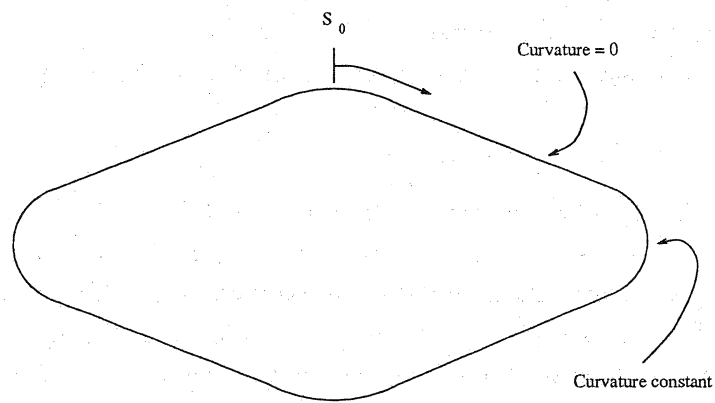
Figure 36: Curvature and 1st and 2nd derivatives
