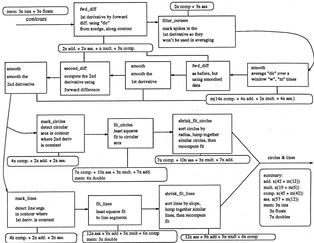
Figure 54: Flowchart of the implemented curvature technique
