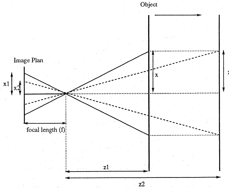
Figure 27: Changing Window Size Assuming Pinhole Camera Model
