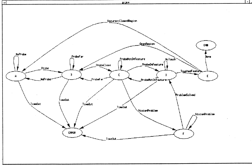
Figure 6: GIIJoe Window w/DRFSM
