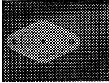
Figure 19: Raw Image
