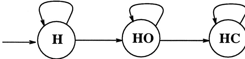
Figure 4: An Automaton for Simple Grasping.
