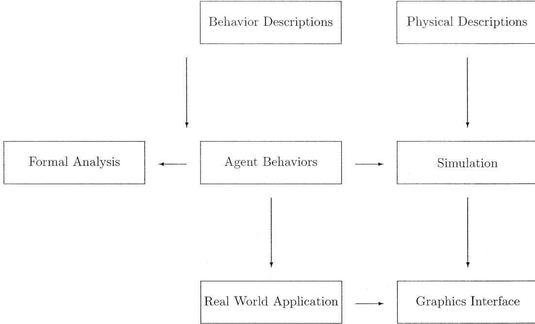
Figure 1: The Z^\infty Framework
