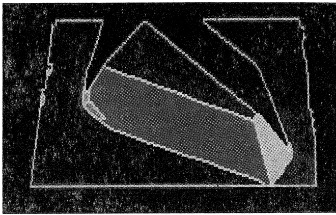
Fig. 13. Planar regions for poly_1.
