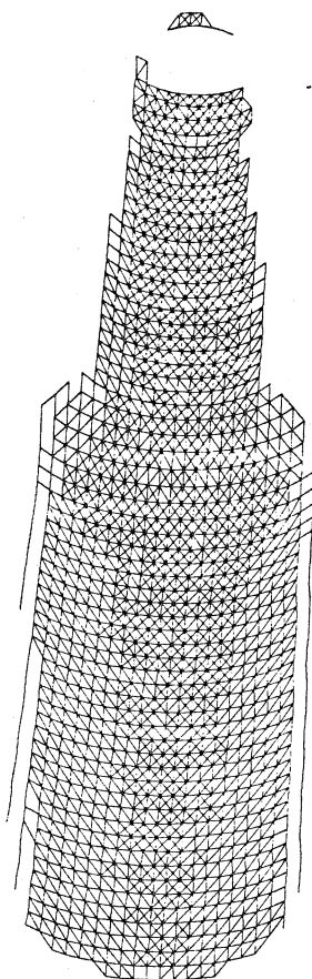
Fig. 18. Bottle spatial proximity graph.
