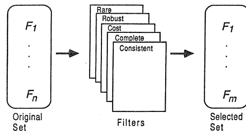
Fig. 2. The feature selection process.
