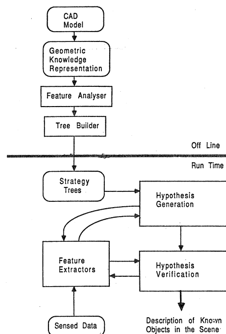
Fig. 3. Overview of strategy trees.
