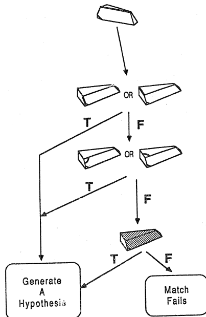
Fig. 9. Corroborating evidence subtree for edge 7.
