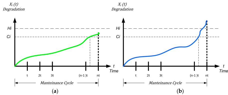
Figure 4. (a) Maintenance limit of preventive maintenance; (b) maintenance limit corrective maintenance.
