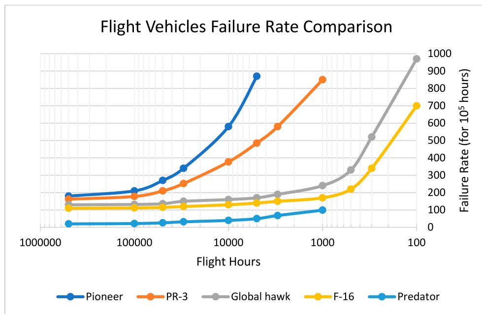
Figure 1. Failure Rate vs. Flight hours for the F-16 and some common drones (figure extrapolated on the data of: Barnard Microsystems Inc. et al. [5]).
