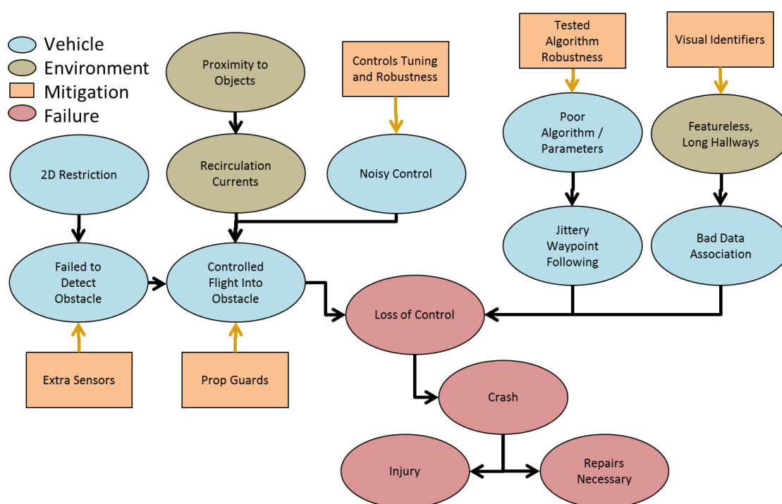
Figure 4: Navigation failure mode graph
