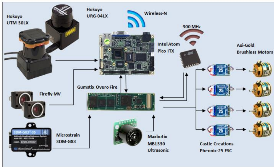
Figure 2: MAAV system architecture
