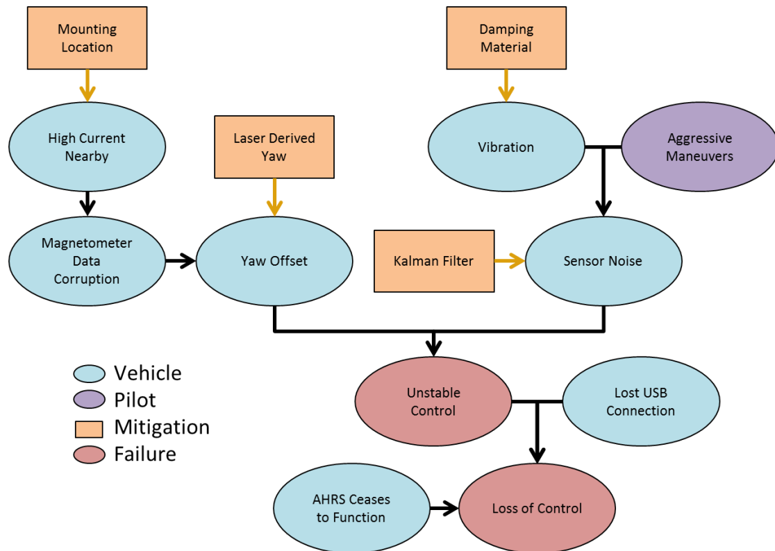
Figure 3: AHRS failure mode graph
