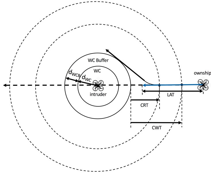
Fig. 1 Structure used in the conflict resolution algorithms
