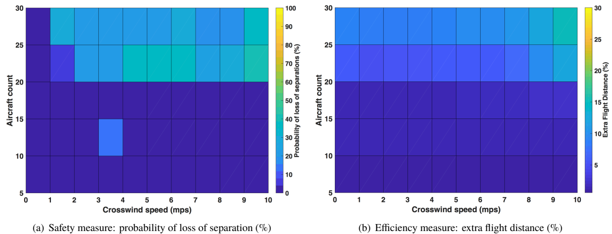
Fig. 5 Impact of Cross Wind on Safety and Efficiency
