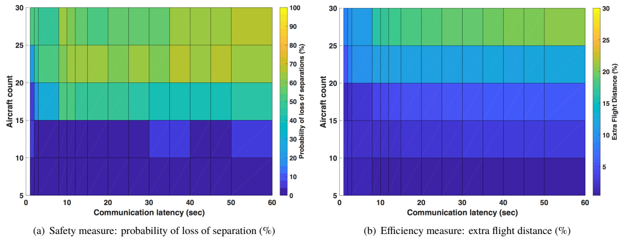
Fig. 4 Impact of Communication Latency on Safety and Efficiency
