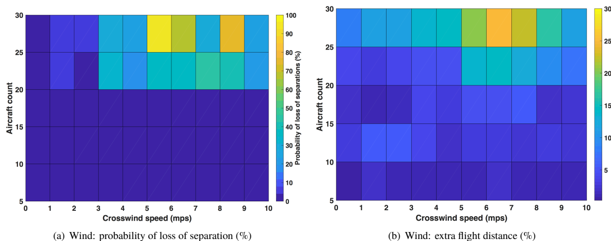
Fig. 8 Impact of Separation Buffer on Safety and Efficiency: Wind
