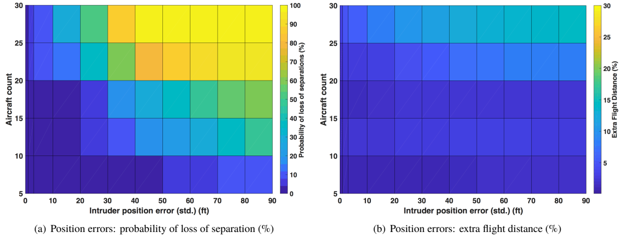
Fig. 6 Impact of Separation Buffer on Safety and Efficiency: Position Errors
