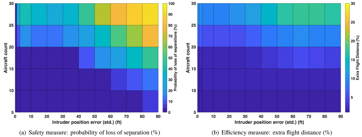
Fig. 3 Impact of Position Errors on Safety and Efficiency
