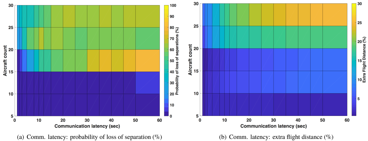
Fig. 7 Impact of Separation Buffer on Safety and Efficiency: Communication Latency
