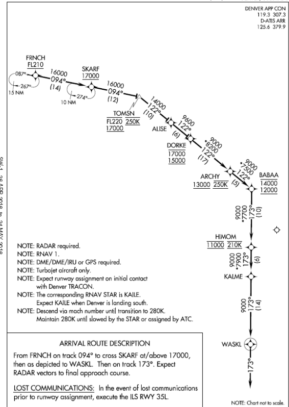
FRNCH THREE ARRIVAL (RNAV) Arrival Route (FRNCH.FRCH3) 18SEP14 DENVER, COLORADO DENVER INTL (DEN)
