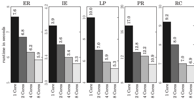
Figure 3: Running time of ROCKIT with CPA on varying number of cores. Due to space considerations we only show the results for the lowest gap 10^{-10} for ER, IE, RC, and PR benchmarks and the gap 0.01 for the LP benchmark.
