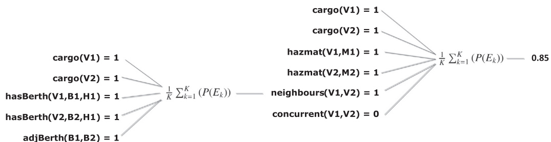
Fig. 9. Example of level of completion calculation for the alarm complex event in formula #15 in Table 12.
