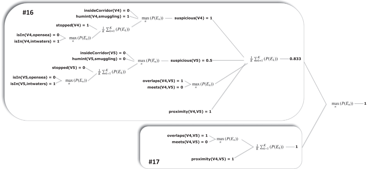
Fig. 10. Example of level of completion calculation for the rendezvous complex event of formulas #16 and #17 in Table 3.
