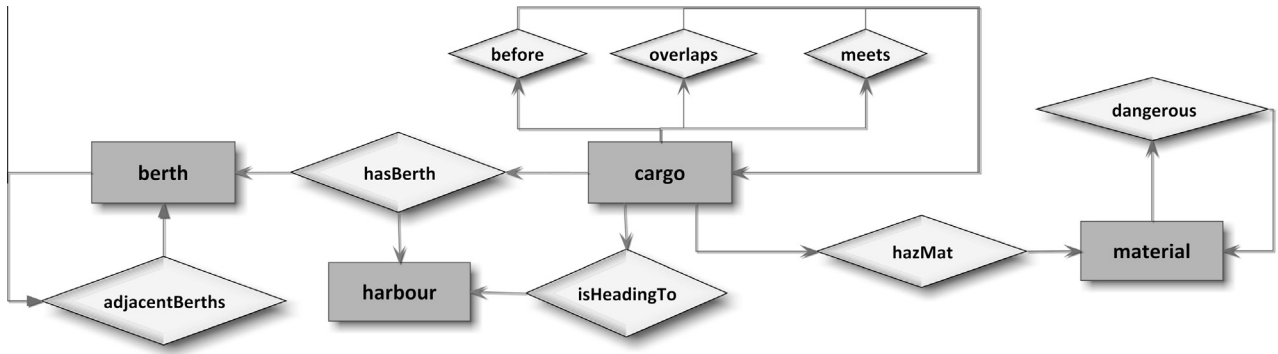
Fig. 7. Entities and relations of the proposed “hazmat” maritime example.
