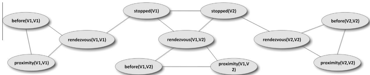
Fig. 4. Example of Markov network. The network is obtained by grounding formulas #18 and #19 in Table 3 with constants V_1 and V_2 referring to two observed vessels.
