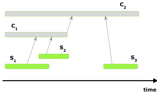
Fig. 2. Example of the detection of a complex event by observing the occurrence of its components. C_2 is composed by complex event C_1 and simple event S_3 . All the events in this example are non-instantaneous as each of them spans a certain interval of time.
