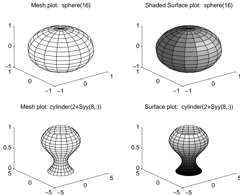
Figure 16: Subplots showing the mesh and shaded surface plots of a sphere determined by three 17 \times 17 matrices of coordinates (named S_{xx} , S_{yy} , and S_{zz} ) and the mesh and surface plots of a cylinder whose width is two plus the y coordinates of the sphere.
