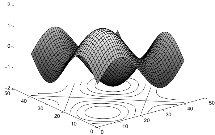
Figure 14: Combined shaded surface plot and contour plot of \sin X + \sin Y .
