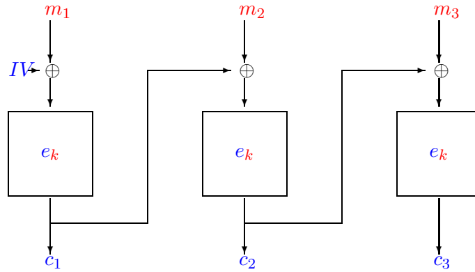
FIGURE 9. CBC encipherment
