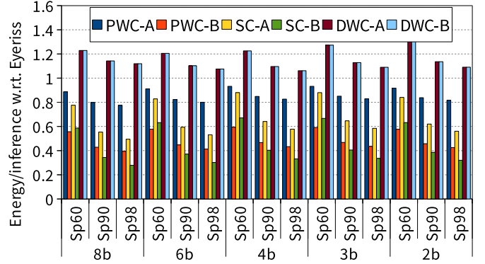
Fig. 14: Energy/inference of SpinalFlow, normalized to an Eyeriss baseline with the same resolution as SpinalFlow. Note that sparsity of Eyeriss is fixed at 60%.
