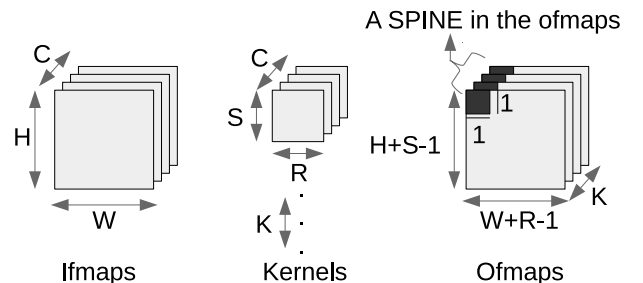
Fig. 6: A spine in a CONV layer.
