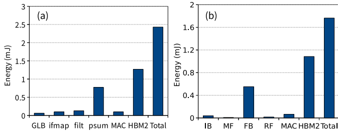
Fig. 12: Energy/inference of ResNet at 8b resolution and 60% sparsity. (a) On Eyeriss, (b) On SpinalFlow. ifmap, filt and psum refers to corresponding scratch-pads in Eyeriss PE.
