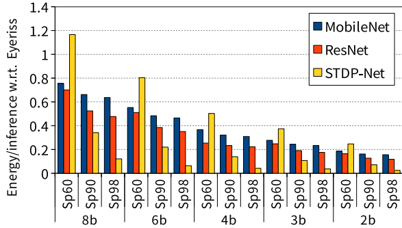
Fig. 13: Energy per inference for SpinalFlow for full workloads, normalized to 8bSp60 Eyeriss.
