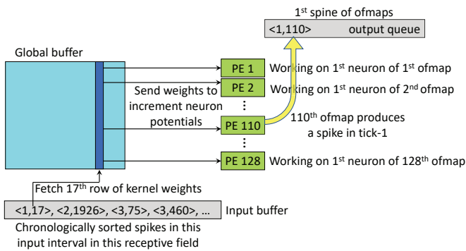
Fig. 7: Example: Step1, Cycle 1.
