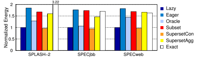
Figure 9. Energy consumed by read and write snoop requests and replies for different algorithms. The bars are normalized to Lazy .
