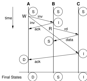
Figure 1. Incorrect execution due to failure to serialize two transactions to the same address.
