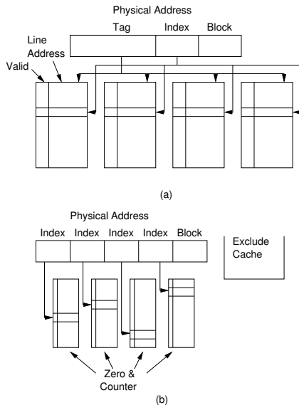
Figure 5. Implementation of the Supplier Predictor.
