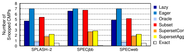
Figure 6. Average number of snoop operations per read snoop request for different algorithms.
