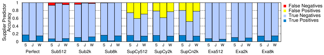
Figure 11. Supplier Predictor accuracy for the different implementations of the Subset , Superset , and Exact algorithms. In the figure, S , J , and W stand for SPLASH-2, SPECjbb, and SPECweb, respectively.
