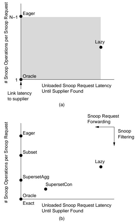
Figure 4. Design space of Flexible Snooping algorithms according to the snoop request latency and the number of snoop operations per request. Chart (a) shows the baseline algorithms, with the shade covering the area of Flexible Snooping algorithms. Chart (b) places the proposed algorithms. The charts assume that one of the nodes provides the line.
