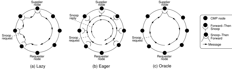
Figure 3. Actions of a snoop request in three different algorithms. Each node is a CMP.
