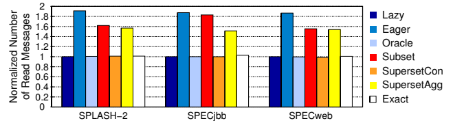
Figure 7. Total number of read snoop requests and replies in the ring for different algorithms. The bars are normalized to Lazy .
