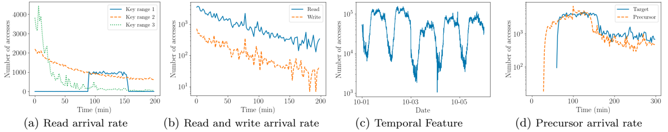
Figure 4: Access patterns in e-commerce scenario. (a) shows read arrival rate of different key ranges have different patterns; (b) shows read arrival rate and write arrival rate of the same key range share similar pattern; (c) shows e-commerce workload has temporal periodicity; (d) shows many key ranges share similar patterns with their precursors.
