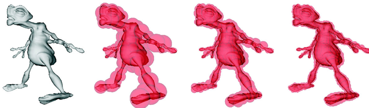
Figure 2.6: Three levels of the sphere tree constructed by Algorithm 2.1.
