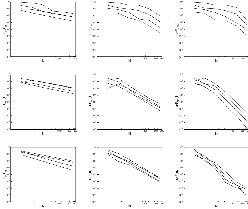
FIGURE 6. Pointwise errors at specific points in the domain as a function of the length of the expansion, N , the order of the filter, p , used in the optimal filter, Eq. (12), and the regularity of the function being approximated. In each figure are four graphs, corresponding to u^{(0)} to u^{(3)} , usually with the former being the top and the latter the bottom graph. The rows corresponds to pointwise errors at x = 0.1 , x = 0.5 , and x = 1.0 , respectively, while the columns reflects p = 2 , p = 6 , and p = 10 .
