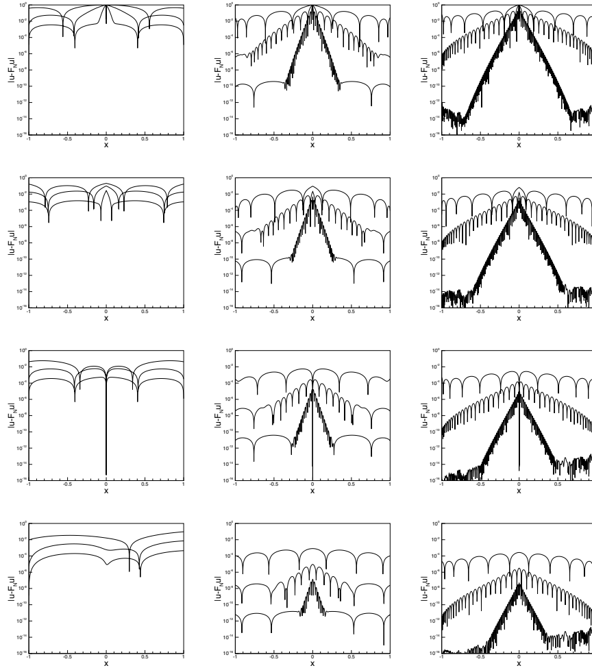
FIGURE 5. In the left column is shown the pointwise error after the exponential filter, Eq. (13), with p = 2 has been applied to the Legendre expansions of the four test functions in Figure 1, with N = 16 , N = 64 and N = 256 , for each function. The middle column shows similar results for p = 6 while the right column displays the results for p = 10 .
