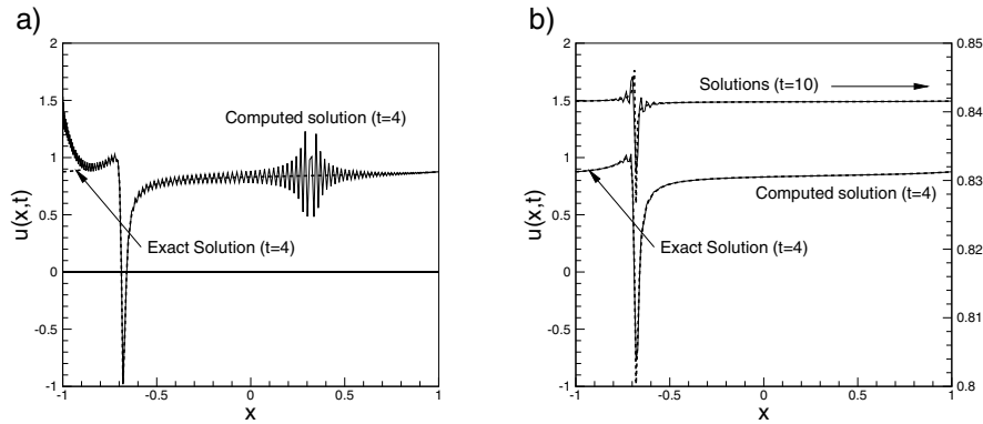
FIGURE 7. In a) we show the exact (dashed line) and computed (full line) solutions to a variable coefficient linear problem at t = 4 . The numerical scheme is a Legendre collocation methods with N = 256 . In b) we show the same problem, however, solved with a weak ( p = 16 ) filter applied. Also shown is the solution at t = 10 .
