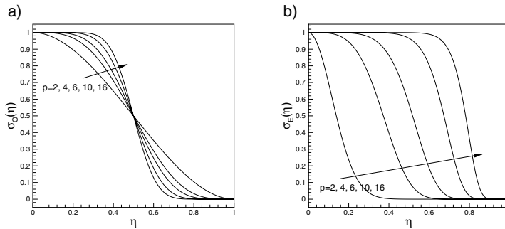
FIGURE 3. In a) we show filter function, \sigma_O(\eta) for the optimal filter, Eq. (12) for increasing values of p . b) shows a similar sequence for the exponential filter, \sigma_E(\eta) , given in Eq. (13).
