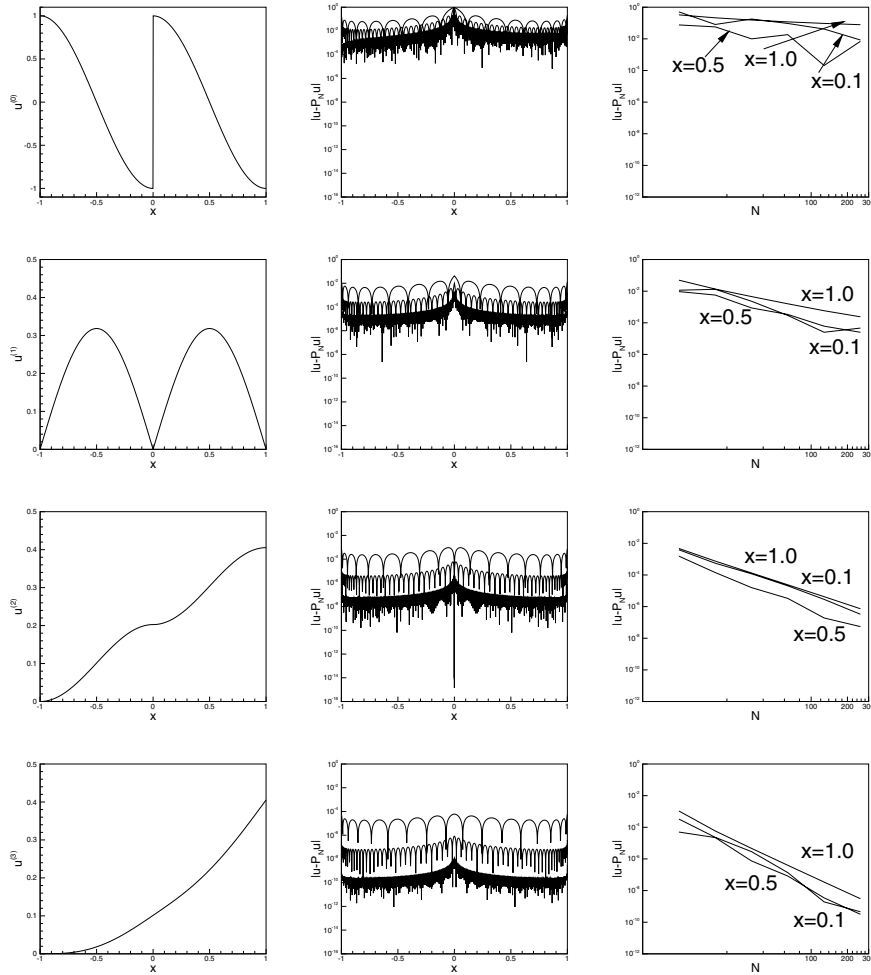
FIGURE 1. The left column shows the first four functions in the sequence, u^{(i)} , defined in Eq. (10). In the middle column we show the pointwise error of the truncated Legendre expansion for each function for increasing values of truncation, exemplified by N = 16 , N = 64 , and N = 256 . In the right column is shown the pointwise error at three points, x = 0.1; 0.5; 1.0 , in the interval.
