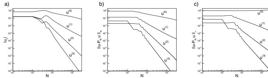
FIGURE 2. In a) we show the envelope, i.e., the upper bound, of |\hat{u}_n| for the first four functions in the sequence, u^{(i)} , defined in Eq. (10). In b) we show the associated L^2 error while c) shows the corresponding L^\infty error.
