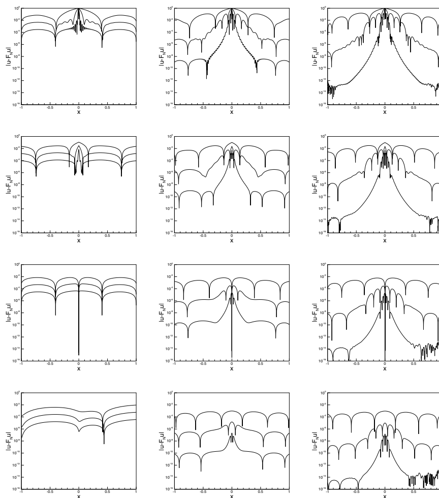
FIGURE 4. In the left column is shown the pointwise error after the optimal filter, Eq. (12), with p = 2 has been applied to the Legendre expansions of the four test functions in Figure 1, with N = 16 , N = 64 and N = 256 , for each function. The middle column shows similar results for p = 6 while the right column displays the results for p = 10 .
