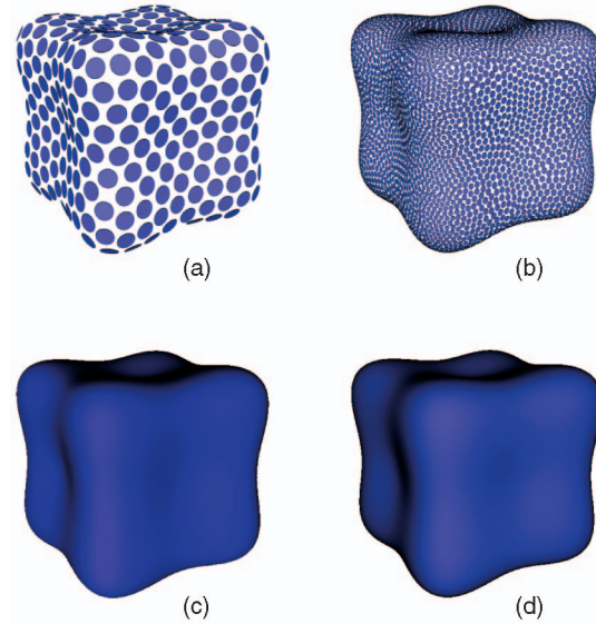
Fig. 10. The zero set of an eighth-order implicit function defined within a single hexahedral element: (a) 500 particles, with a distribution time of 4 seconds, (b) 6,800 particles, with a distribution time of 3 minutes, and (c) a GPU-based splat rendering of the 6,800 particles that is visually indistinguishable from the 512 \times 512 ray traced image in (d).
