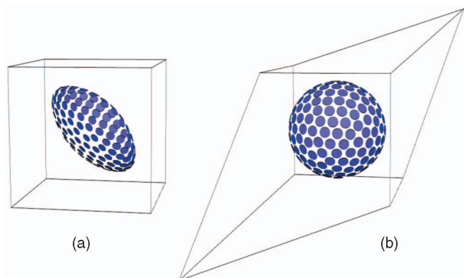
Fig. 8. (b) The particle system converges to an even distribution in world space regardless of (a) the shape of the surface in reference space.
