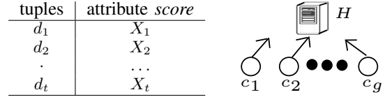
Fig. 2. Attribute-level uncertain tuple and the flat model.
