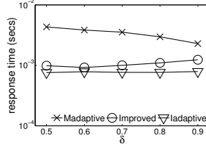
Fig. 10. Response time: vary \delta
