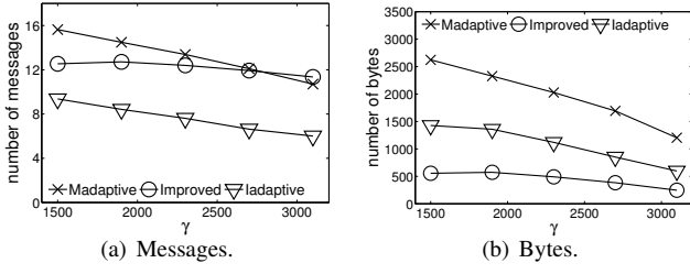
Fig. 8. Communication: vary \gamma .
