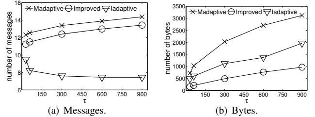
Fig. 15. Communication: vary \tau .
