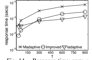
Fig. 14. Response time: vary \tau
