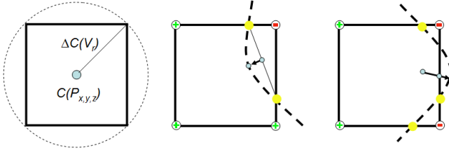
Figure 2: (a) A 2D illustration of a cell being tested for a possible solution using the cell radius as a bound on changes to the constraint value. (b) A solution point is found by finding zero crossing (in yellow) along edges. The average of these points provides an initial guess which then moves onto the solution set. (c) Some mass points provide poor initial guesses, and the solution point is clipped to remain in the cell bounds.
