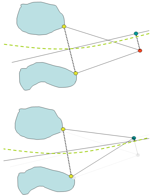
Figure 7: Projecting the mass point onto the linear bisector of the two closest points on the models geometrically converges the mass point onto the true bisector manifold. The true bisector manifold is shown as a dashed line.
