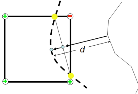
Figure 3: Points on the offset manifold are found by computing the closest point on the surface and using the surface normal at that point to move the cell's mass point onto the constraint zero set.
