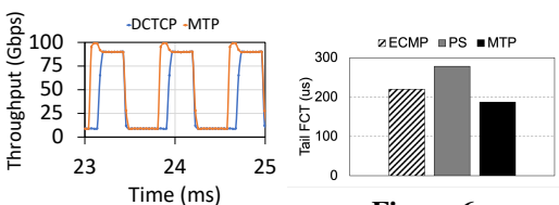
Figure 5: Multi-path CC
