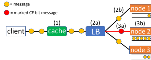
Figure 1: A network that benefits from in-network computing
