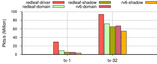
Figure 7: Software-only nullnet driver performance
