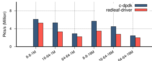
Figure 10: Key-value store
